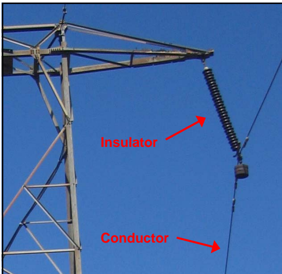
Top of lattice steel tower illustrating insulator and conductor.
